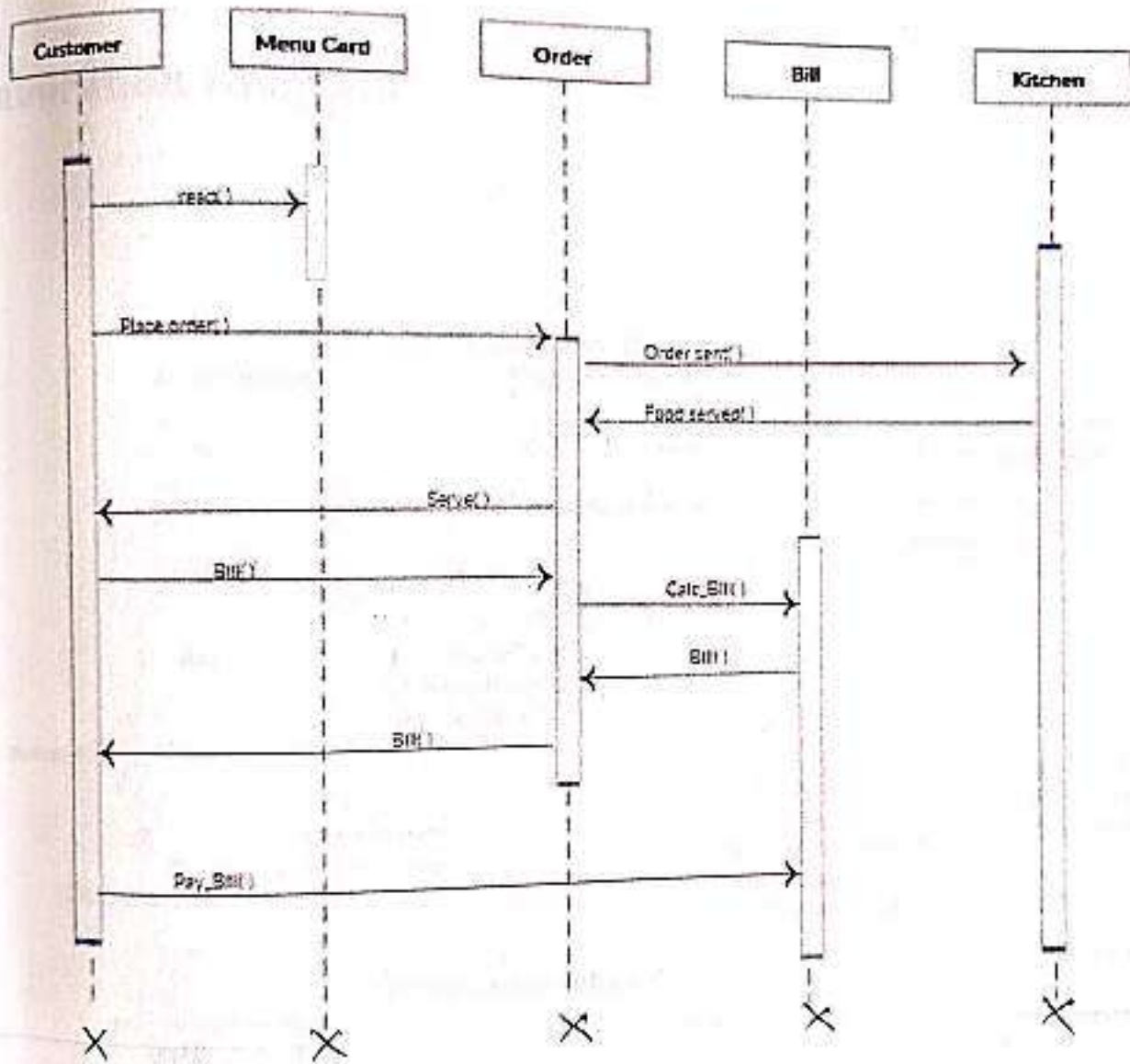
SEQUENCE DIAGRAM FOR FOOD ORDERING SYSTEM
